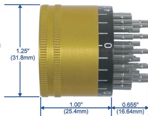
48DF-1/2 (Female)
