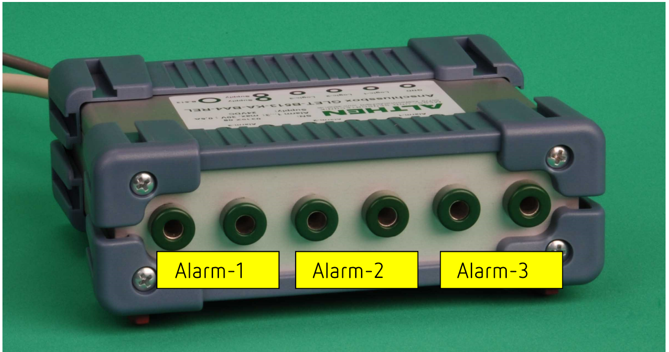
Alarm 1: N/O
