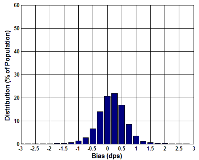
Figure 5.16 Analogue Bias (dps) at -40°C
