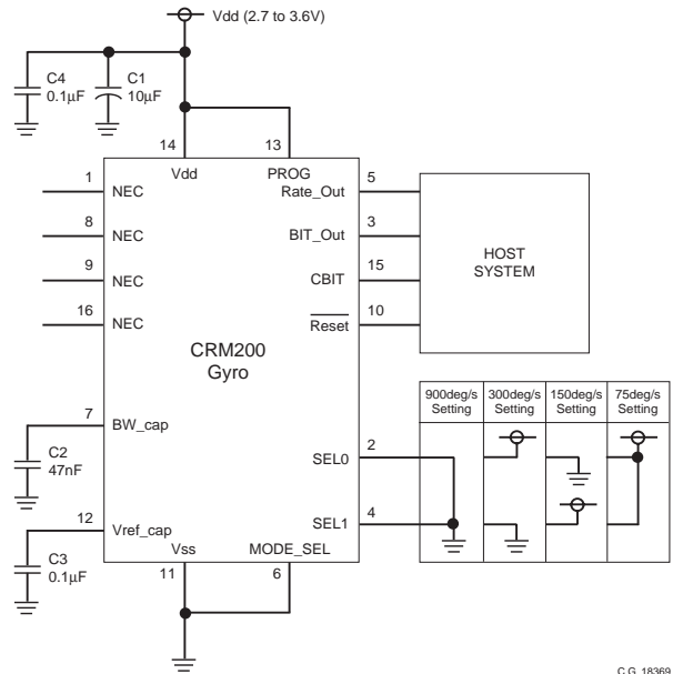
Figure 7.3 Peripheral Circuit - Analogue Output (CRM200)
