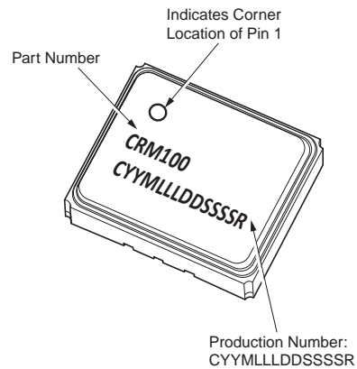
Figure 11.1 Part Marking
