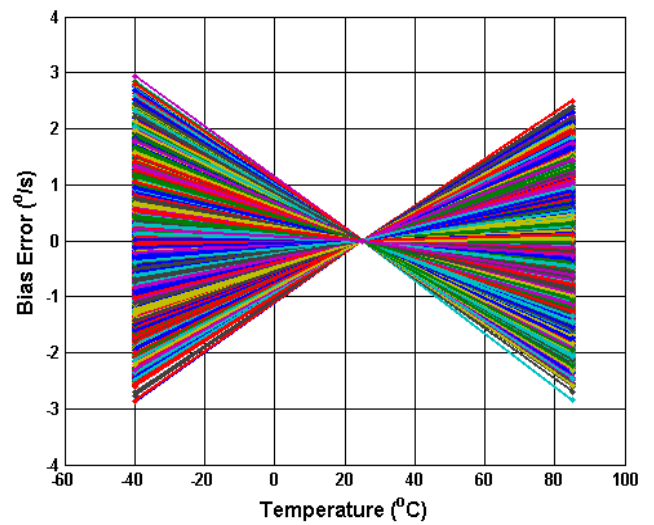
Figure 5.3 Analogue Normalised Bias Error (dps) vs Temperature
