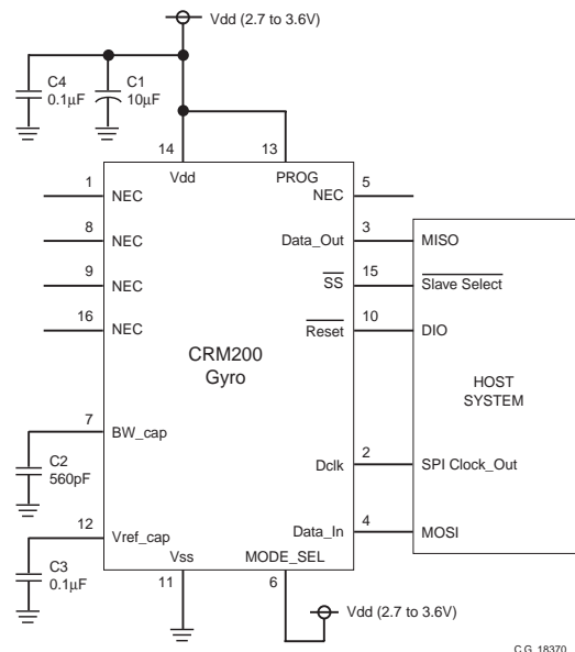
Figure 7.4 Peripheral Circuit - Digital Output (CRM200)
