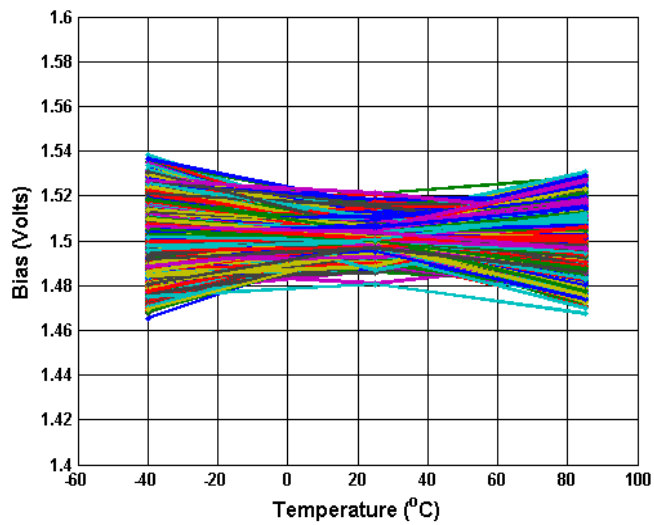
Figure 5.1 Analogue Bias (Volts) vs Temperature
