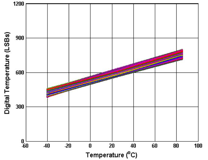
Figure 5.27 Digital Temperature Output (LSB) vs Temperature
