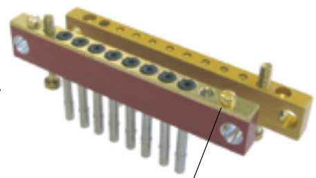
Screws supplied with gasstage to fasten gasstage to one half of the connector.
