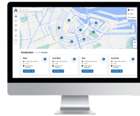
SmartBrick Dashboard
